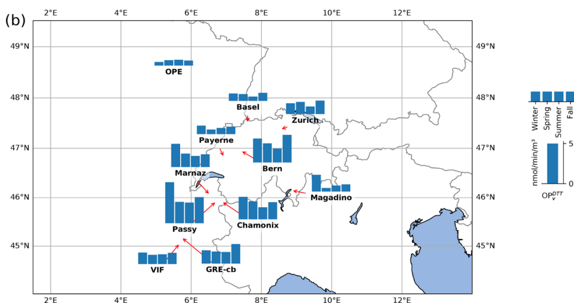
Figure 2. Seasonal volumetric OP^{DTT} means for the five Swiss sites included in this analysis and the closest six French sites surrounding Switzerland. Data from the French sampling sites are from Weber et al. (2021) and Grange et al. (2022).
