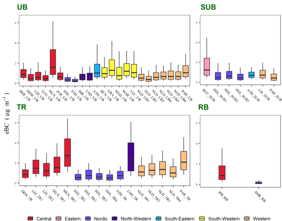
Figure 2. Variability of averaged eBC mass concentrations at 50 sites between 2017 and 2019 categorized by the type of site and region. Modified from Savadkoohi et al. (2023).
