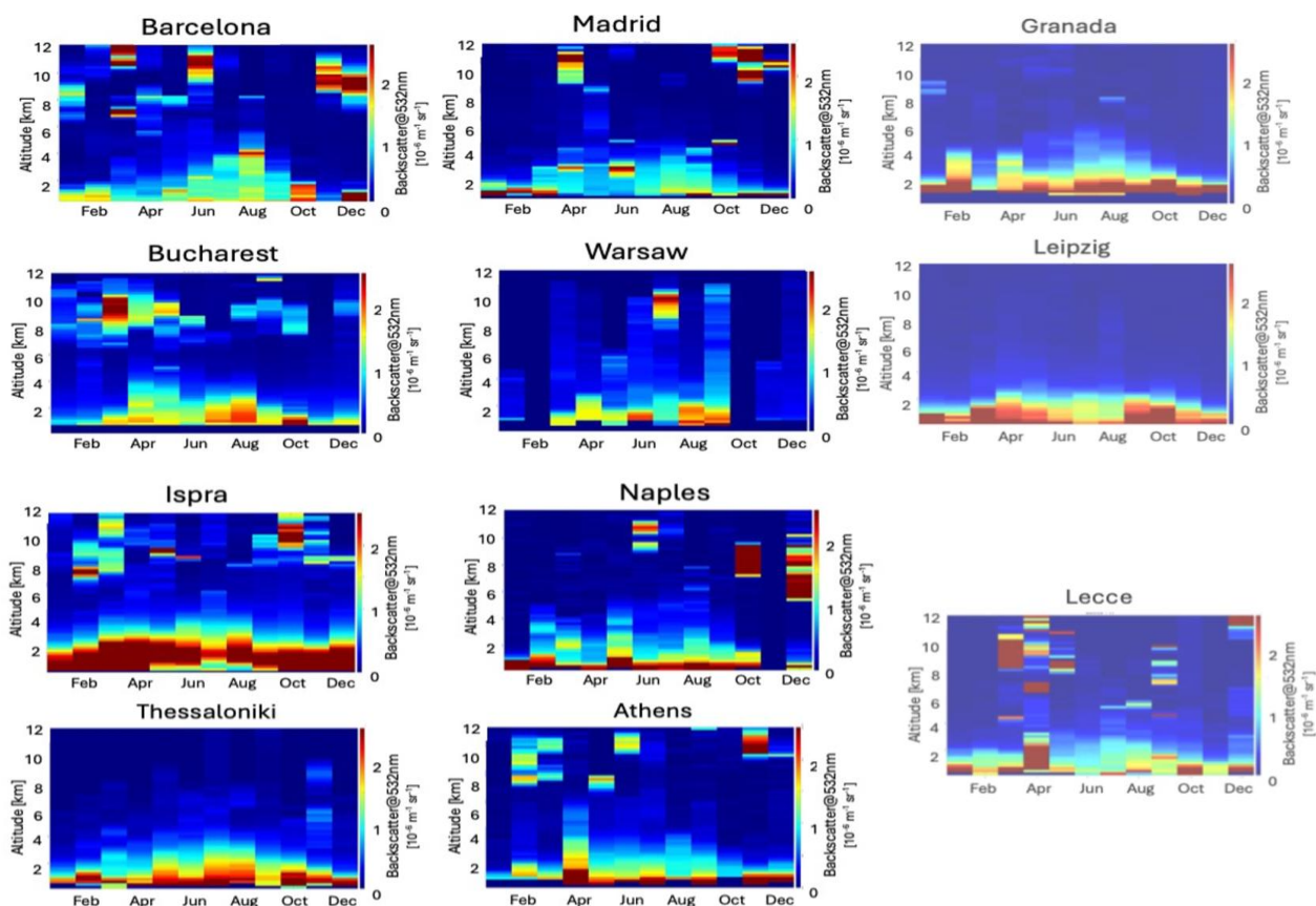
Figure 3: Climatological monthly averages of the aerosol backscatter profile at 532 nm in suburban locations close by 8 big cities: Barcelona, Madrid, Bucharest, Warsaw, Ispra, Naples, Thessaloniki and Athens. In the third column the same quantity is reported, as partially transparent, for 3 sites far from big cities located in the same macro-area of the previous reported 8 ones.
