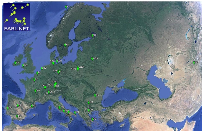
Figure 2. ACTRIS/EARLINET stations included for which Level 3 climatology is available.
