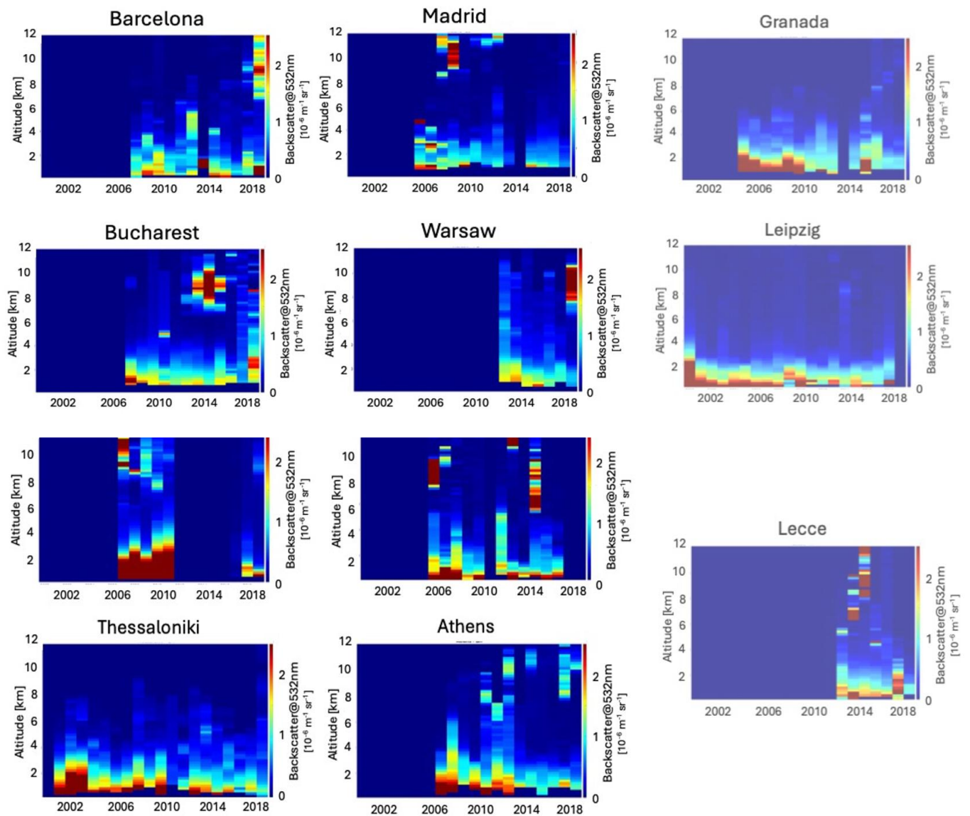
Figure 4. Annual averages in the period 2000-2019 of the aerosol backscatter profile at 532 nm in suburban locations close by 8 big cities: Barcelona, Madrid, Bucharest, Warsaw, Ispra, Naples, Thessaloniki and Athens. In the third column the same quantity is reported, as partially transparent, for 3 sites far from big cities located in the same macro-area of the previous reported 8 ones.
