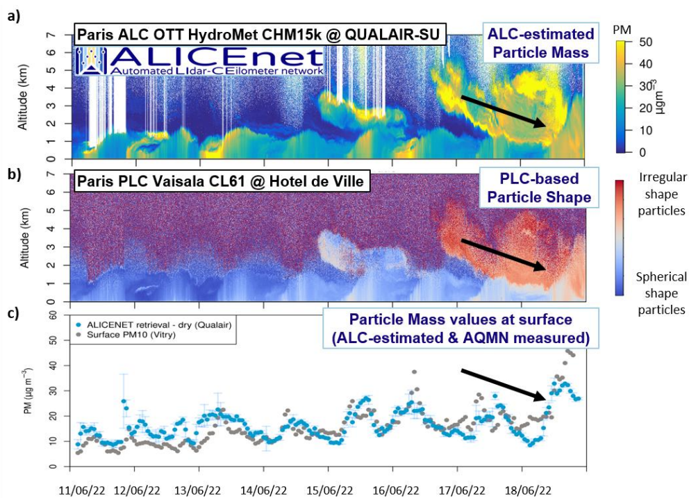
Figure 1. Example of application of ALICENet methods upscaling over the RI-URBANS Paris Pilot site during a desert dust event in June 2022. Vertical (0 -7 km, y axis) and temporal (June 11-18, x axis) evolution of (a) particle mass vertical profiles, and (b) particle shape; (c) temporal (June 11-18, x axis) evolution of particle mass values at the ground as derived from in situ PM10 measurements (grey dots) and ALC at surface-level (adapted from Bellini et al., 2025, in preparation).
