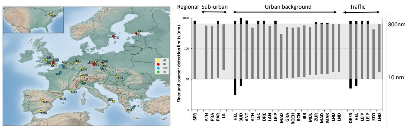
Figure 1: Left: Location of the cities supplying data on particle number concentrations and size distributions for the present study and the type of station. UB, Urban background; TR, Traffic; SUB, Suburban background; RB, Regional background. Right: Particle size detection limits of PNSD measurements of this study and recommended ones from CEN (10–800 nm). Modified from Trechera et al. (2023).
