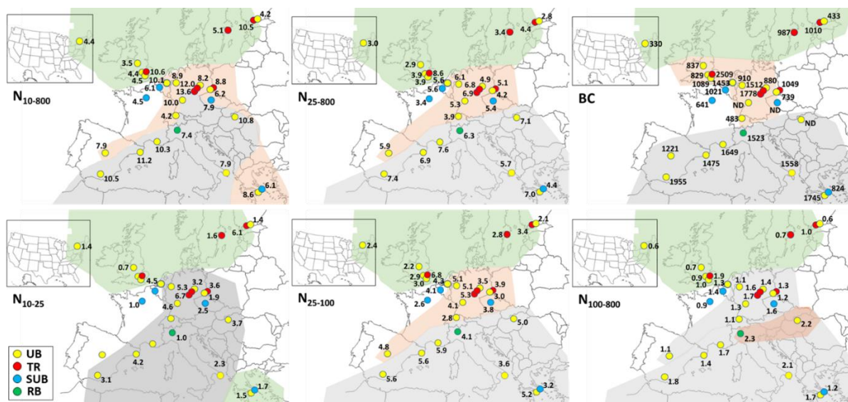
Figure 3: Regional variability of averaged 2017-2019 particle number concentrations (in \text{# cm}^{-3} 10^{-3} ) size fractions (in \text{# cm}^{-3} 10^{-3} ) and black carbon (BC in \text{ng m}^{-3} ) in Europe. For N_{10-25} , only sites with a lower size detection limit of 10-14 \text{ nm} are included. UB, Urban background; TR, traffic; SUB, Suburban background; RB, Regional background. Modified from Trechera et al. (2023).
