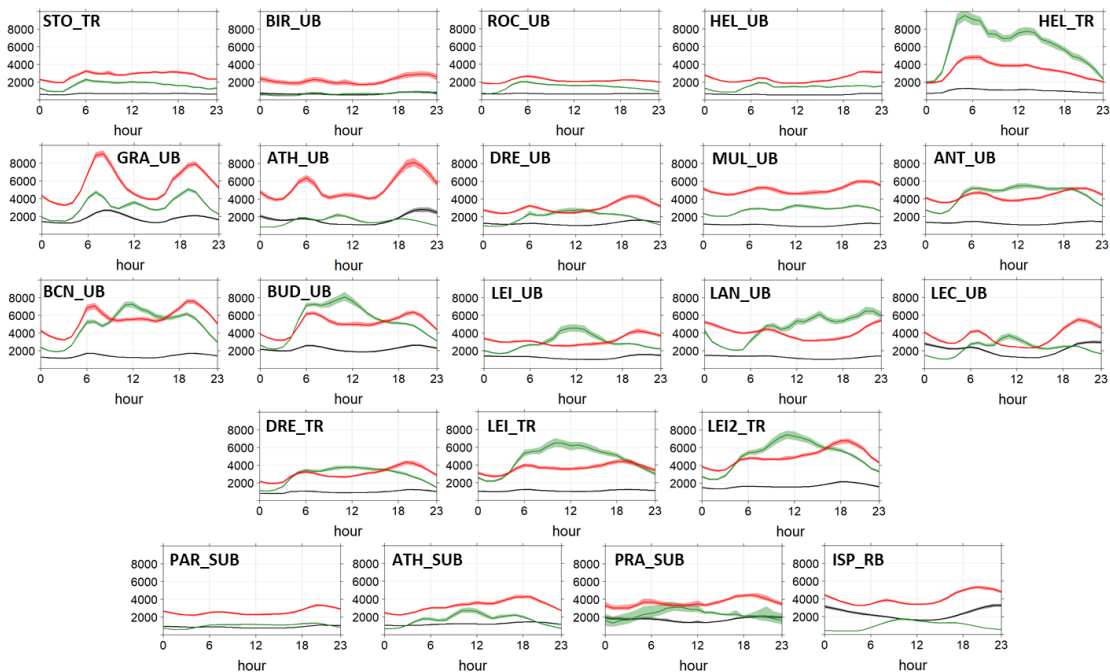
Figure 5: Averaged 2017-2019 hourly concentrations of the particle number fractions (in # cm -3 ) N 10-25 (green), N 25-100 (red) and N 100-800 (grey). Only sites with a lower size detection limit of 10-14 nm are included. UB, Urban background; TR, Traffic; SUB, Suburban background; RB, Regional background. Modified from Trechera et al. (2023).
