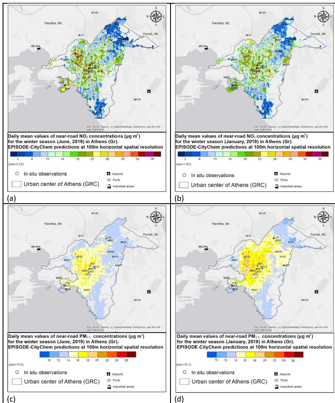
Figure 2. NO 2 [(a) and (b)], PM 2.5 [(c) and (d)], near-road concentrations (µg m -3 ) over Athens simulated for summer (left panels) and winter (right panels) using EPISODE-CityChem.
