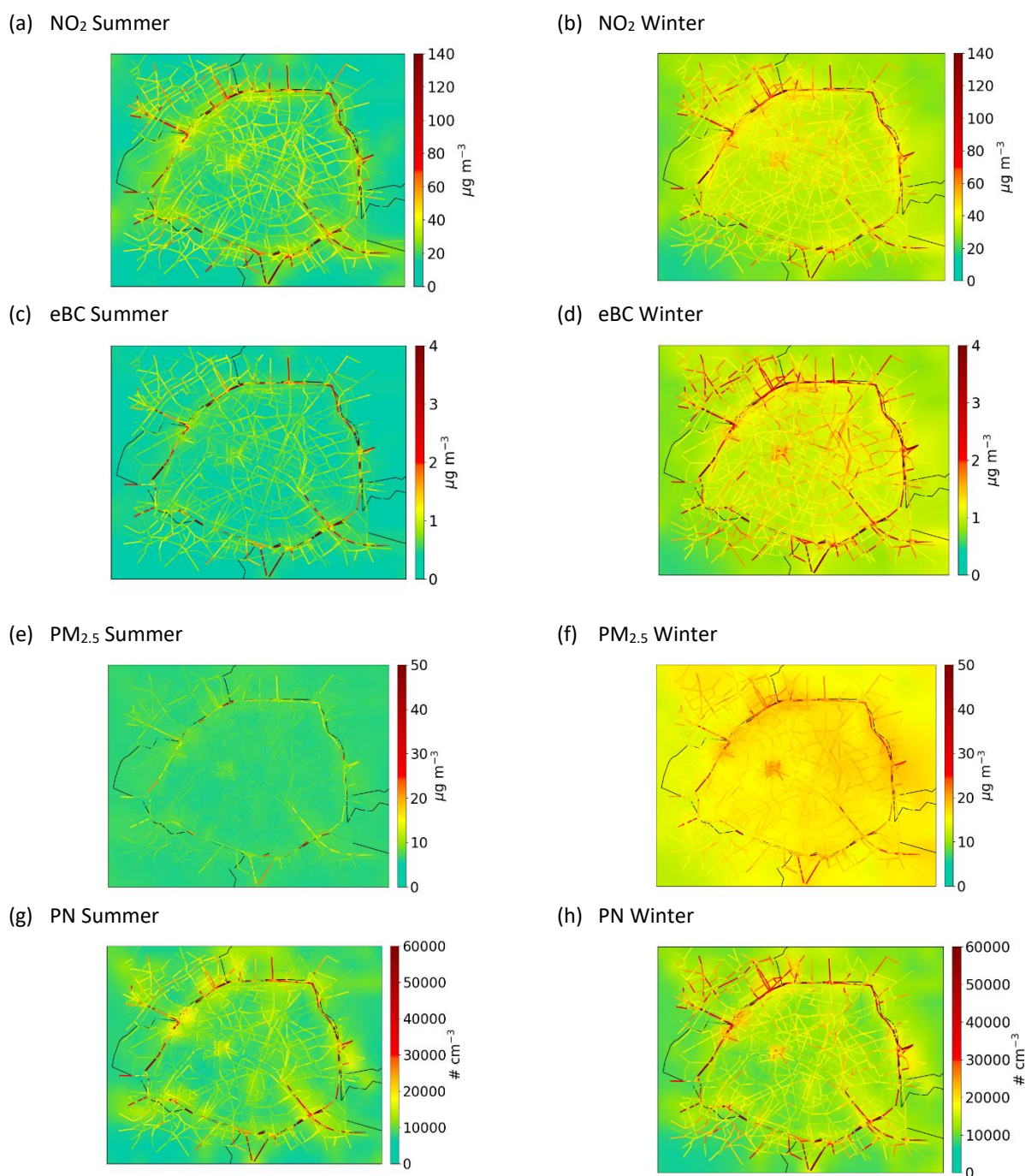
Figure 1. NO 2 [(a) and (b)], BC [(c) and (d)], PM 2.5 [(e) and (f)], and PNC [(g) and (g)] concentrations simulated for summer (left panels) and winter (right panels) using CHIMERE/MUNICH.
