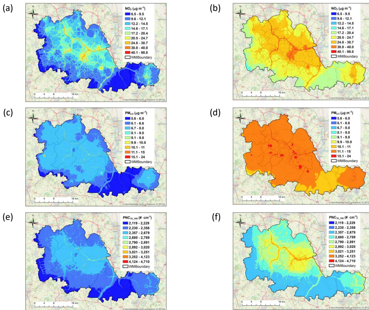
Figure 3. NO 2 [(a) and (b)], PM 2.5 [(c) and (d)], and PNC [(e) and (f)] concentrations simulated for Summer (left panels) and Winter (right panels) using ADMS-Urban.
